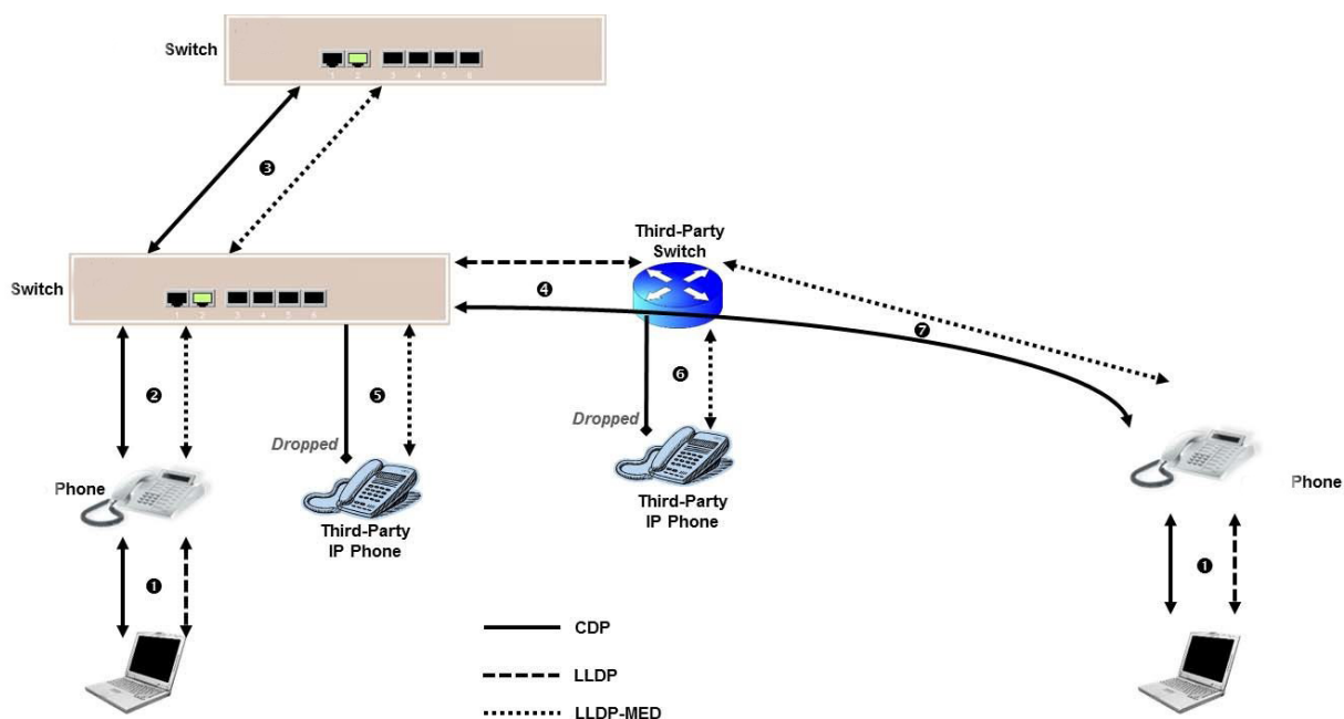
Figure CDP Operations
