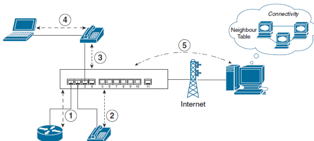
Figure LLDP Operations
